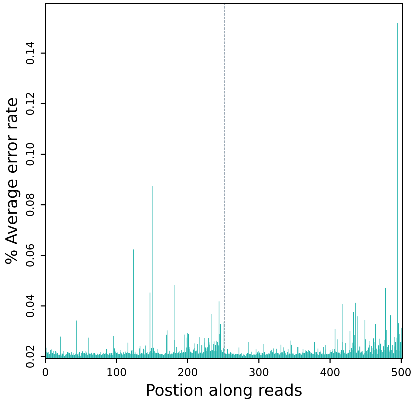
Error rate distribution along reads (R10326)
